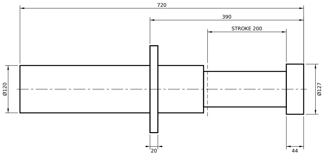
FRONT FLANGE MOUNT (FF)
