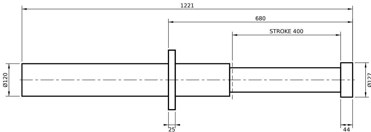
FRONT FLANGE MOUNT (FF)
