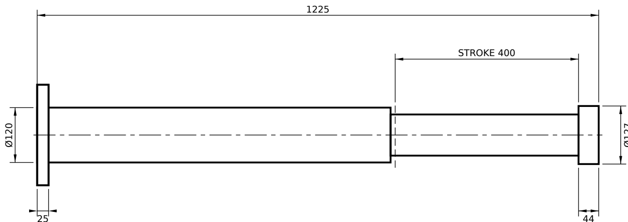
REAR FLANGE MOUNT (FR)
