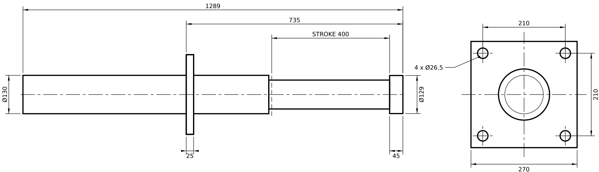
FRONT FLANGE MOUNT (FF)
