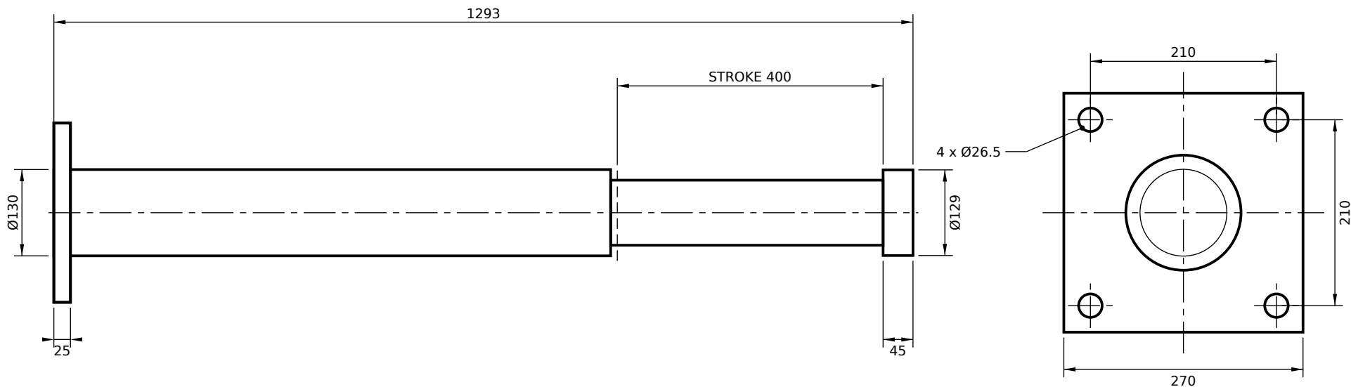
REAR FLANGE MOUNT (FR)
