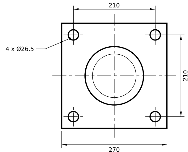
VIEW FROM ROD END (SCALE 1:6)
