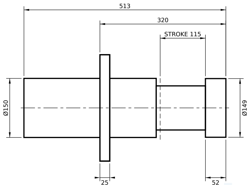
FRONT FLANGE MOUNT (FF)
