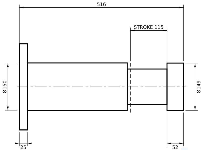
REAR FLANGE MOUNT (FR)
