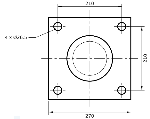
VIEW FROM ROD END
