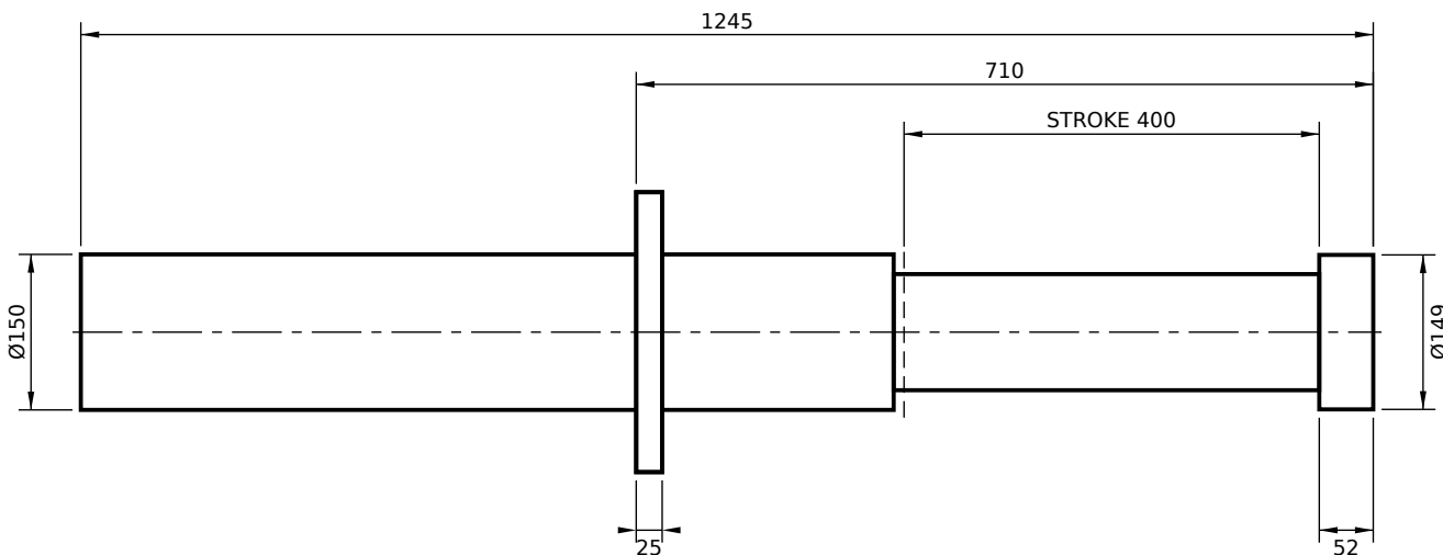
FRONT FLANGE MOUNT (FF)
