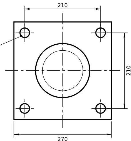
VIEW FROM ROD END (SCALE 1:6)
