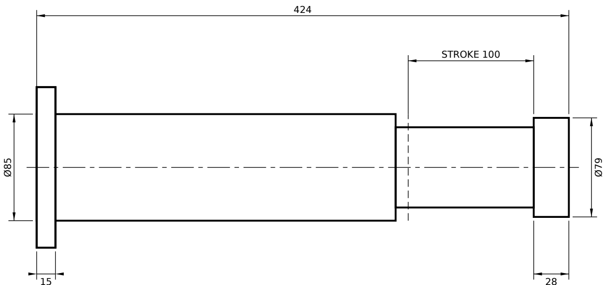
REAR FLANGE MOUNT (FR)
