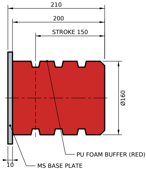
PU BUFFER - BASE PLATE MOUNT
