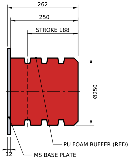
PU BUFFER - BASE PLATE MOUNT
