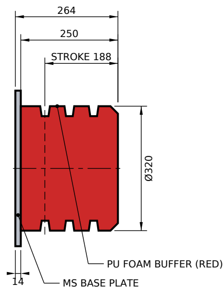
PU BUFFER - BASE PLATE MOUNT
