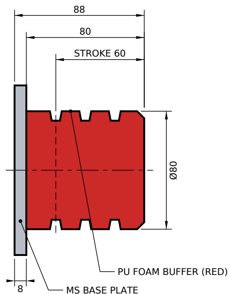
PU BUFFER - BASE PLATE MOUNT
