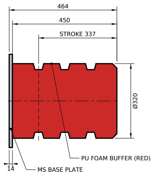
PU BUFFER - BASE PLATE MOUNT
