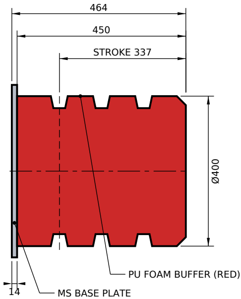
PU BUFFER - BASE PLATE MOUNT
