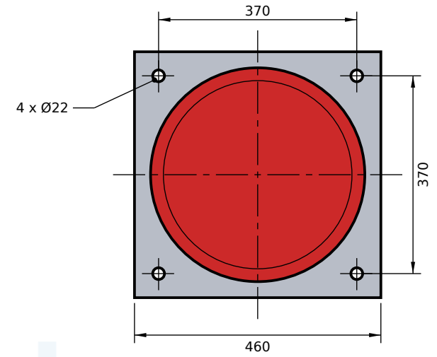
VIEW FROM STRIKER END
