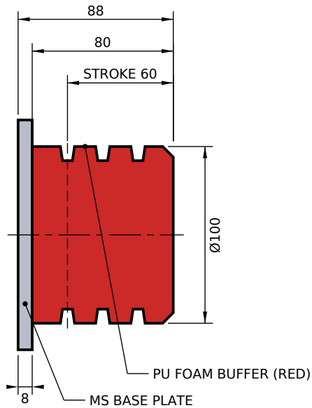
PU BUFFER - BASE PLATE MOUNT
