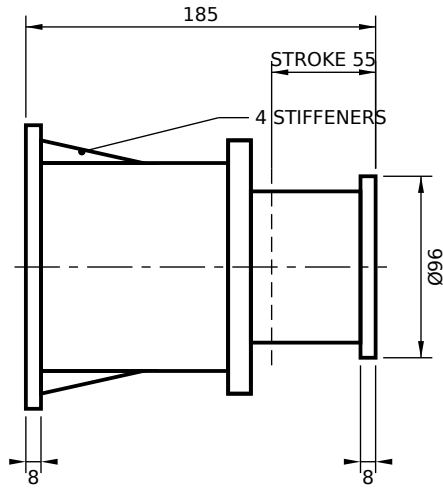
SPRING BUFFER - BASE PLATE MOUNT
