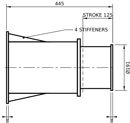
SPRING BUFFER - BASE PLATE MOUNT
