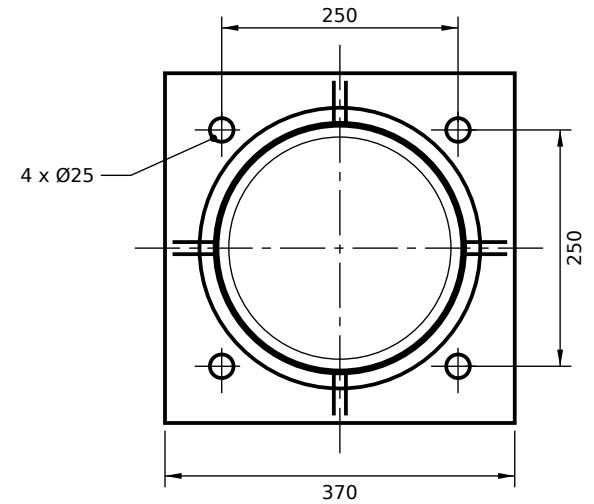
VIEW FROM STRIKER END (SCALE 1:8)
