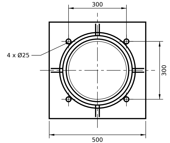
VIEW FROM STRIKER END
