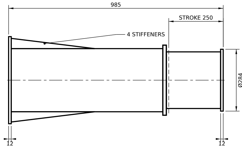
SPRING BUFFER - BASE PLATE MOUNT
