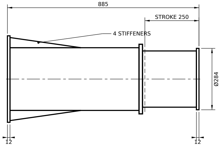
SPRING BUFFER - BASE PLATE MOUNT
