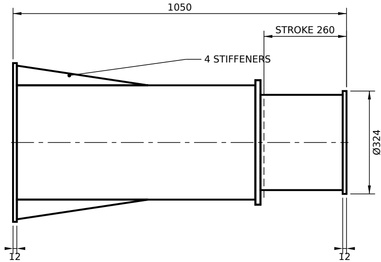
SPRING BUFFER - BASE PLATE MOUNT
