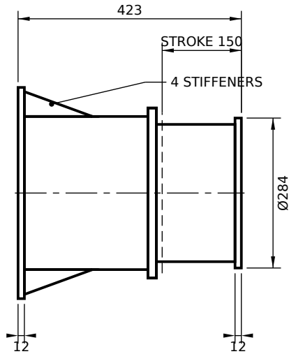
SPRING BUFFER - BASE PLATE MOUNT
