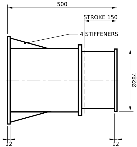
SPRING BUFFER - BASE PLATE MOUNT
