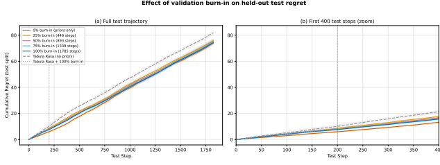
Figure 10: Validation burn-in ablation—unconstrained (K=3 stationary, 20 seeds, 95% bootstrap CI, held-out test split). Left: cumulative regret on test under varying burn-in fractions (0–100% of val). All warmup conditions are statistically indistinguishable ( p > 0.15 ); the only significant gap is tabula rasa without burn-in (+10.0%, p < 10^{-5} ). Right: zoom on the first 400 test steps—0% burn-in (priors only) has the lowest early regret because priors are fully intact.
