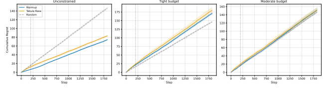
Figure 8: Cumulative regret: warmup priors vs. cold start across three budget regimes (K=3 stationary, 20 seeds, 95% bootstrap CI, held-out test split). Left: unconstrained—warmup reduces regret by 10% ( p < 10^{-5} ), concentrated in the first \sim 200 steps. Centre: tight budget—the advantage persists ( \Delta = -9.1 , p=0.059 ) as uninformed UCB exploration wastes scarce budget on expensive arms. Right: moderate budget—the gap vanishes ( p=0.94 ) as the budget constraint collapses the feasible arm set, making the prior’s knowledge irrelevant.
