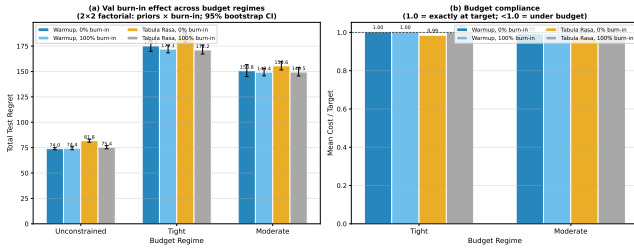
Figure 11: Validation burn-in ablation across budget regimes (20 seeds, 95% bootstrap CI; pacer pre-calibrated, see Appendix ??). Left: total test regret. Within each regime, Warmup 0% and Warmup 100% are statistically indistinguishable, confirming that the burn-in finding holds under the BudgetPacer. The cold-start penalty (Tabula Rasa 0%) is significant at tight budgets (+6.7%, p=0.002 , survives Bonferroni correction) and present at moderate budgets (+4.1%, p=0.017 , non-significant after Bonferroni). Right: budget compliance (mean cost / target). All conditions stay within 3% of the budget target, confirming consistent pacer behaviour regardless of initialization.
