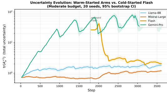
Figure 15: Uncertainty evolution during model onboarding (moderate budget, 20 seeds, 95% bootstrap CI). \text{tr}(A_t^{-1}) measures total uncertainty per arm: higher values indicate less information and larger exploration bonuses. Warm-started arms (Llama-8B, Mistral-Large) maintain low, stable uncertainty ( \sim 0.6 – 2 ) throughout both phases. Cold-started Flash appears at the Phase 2 boundary with \text{tr}(A_t^{-1}) = d/\lambda = 26 (the isotropic prior A = \lambda I ) and converges to the incumbents' level within \sim 300 steps as LinUCB's exploration bonus drives traffic to it. Gemini-Pro exhibits rising, oscillatory uncertainty because it is rarely selected under budget pressure—geometric forgetting erases its accumulated information faster than new observations replenish it, illustrating the forgetting–budget pacer feedback loop described in Section 4.
