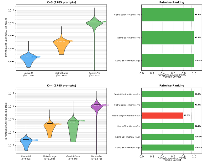
Figure 16: Cost heuristic validation. Left: violin plots of actual per-request costs (log scale) for each model, ordered by the static heuristic \tilde{c}_a . Right: fraction of prompts where each pairwise cost ordering matches the heuristic ranking. Top row: K=3 portfolio; bottom row: K=4 with Gemini-Flash added.
