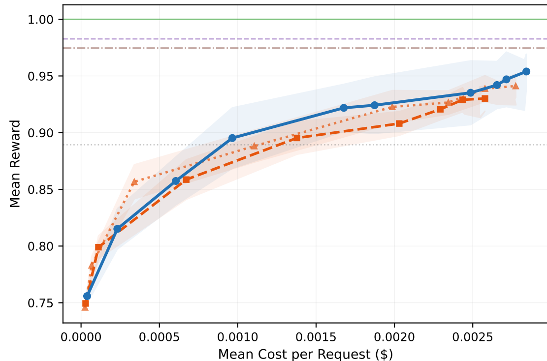
K=5 Portfolio
