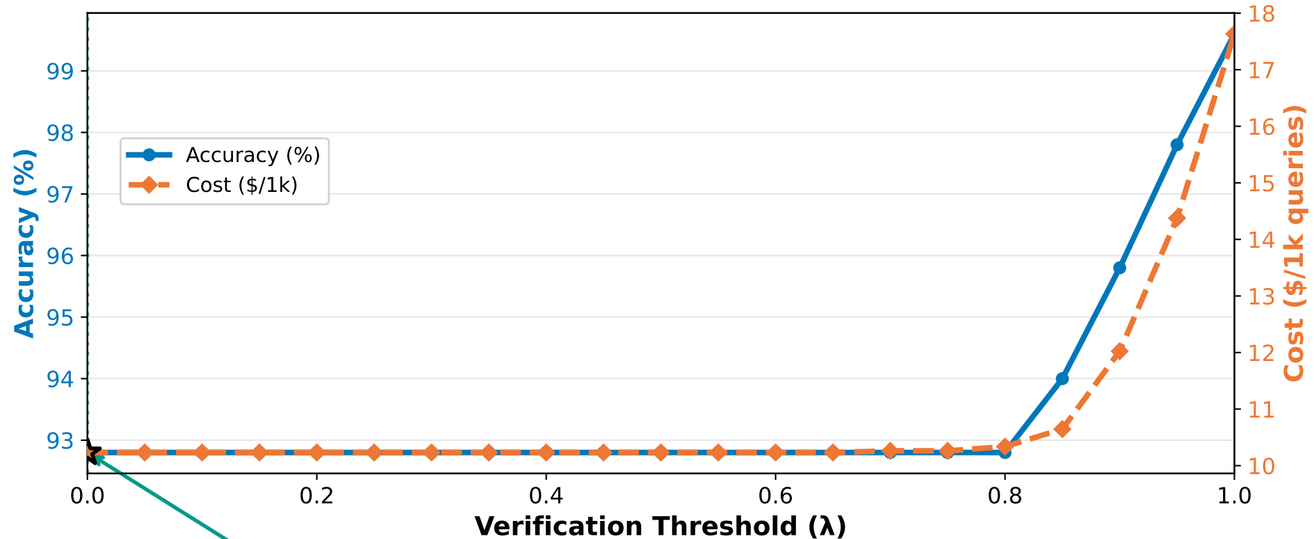
Figure 7: Dialing the Pareto Frontier (Real Model Data) Users dynamically trade cost for accuracy via verification threshold
