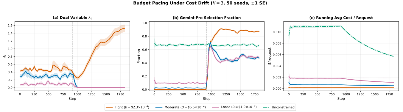
Figure 5: BanditGPT dual-variable dynamics under a mid-stream Gemini price drop (step 912; 50 seeds, \pm 1 SE). (a) The dual variable \lambda_t reveals qualitatively distinct responses: at tight budget, \lambda_t rises because costs still exceed the target (binding constraint); at moderate/loose budgets, \lambda_t decays to zero as post-drop costs fall well below target (slack constraint). (b) Gemini selection fraction mirrors the dual signal—tight budget drives 87% Gemini adoption via cost-penalty concentration; moderate/loose converge toward the unconstrained baseline (dash-dot). (c) Running average cost per request; dotted lines mark budget targets. All three regimes exhibit the correct Lagrangian response. Quantitative compliance comparisons with baselines are in Table ??.
