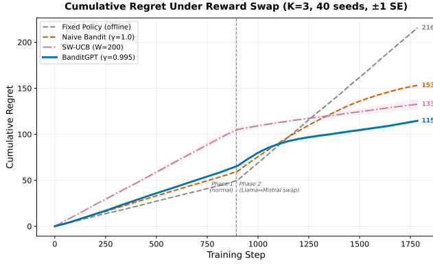
Figure 4: Cumulative regret under reward drift (4 conditions, 40 seeds, \pm 1 SE). BanditGPT ( \gamma=0.995 ) achieves the lowest total regret by combining warmup priors (low Phase 1 cost) with geometric forgetting (fast Phase 2 adaptation). SW-UCB adapts fastest post-shift but pays a large cold-start tax.
