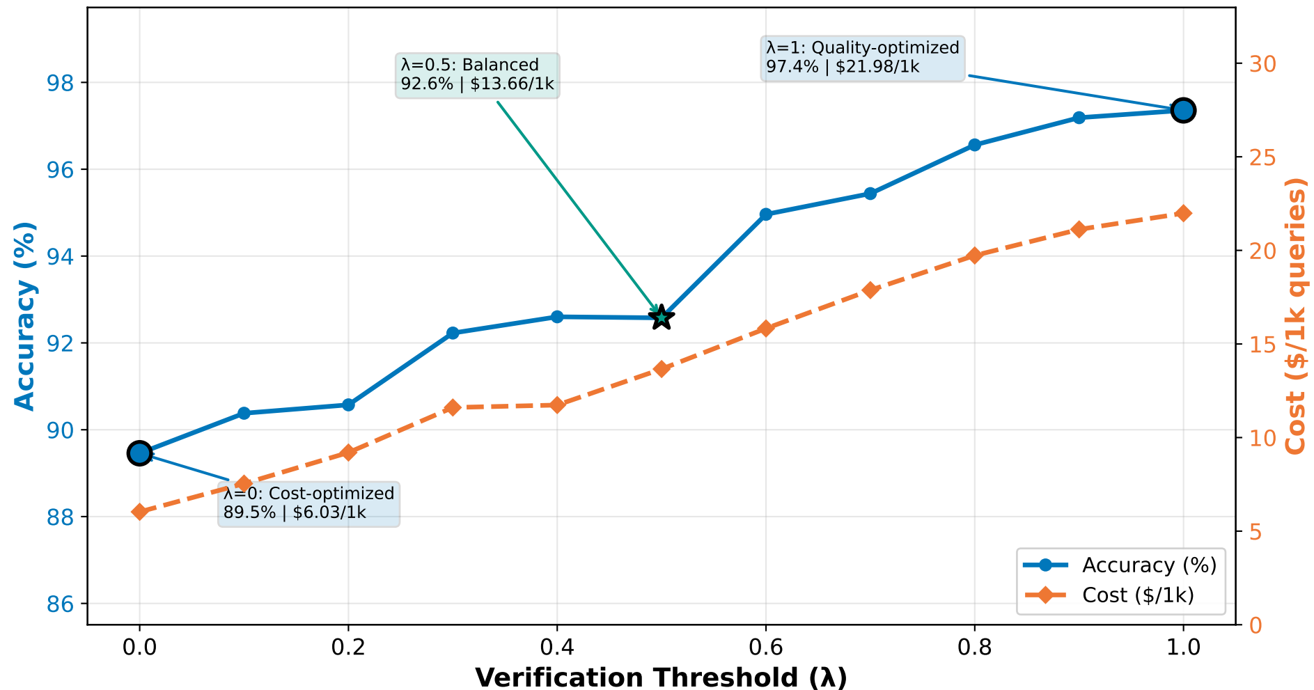
Figure 7: Dialing the Pareto Frontier (Actual HybridRouter) cascade_rate ( \lambda ) controls verification frequency: 0=Standard, 1=Always Verify
