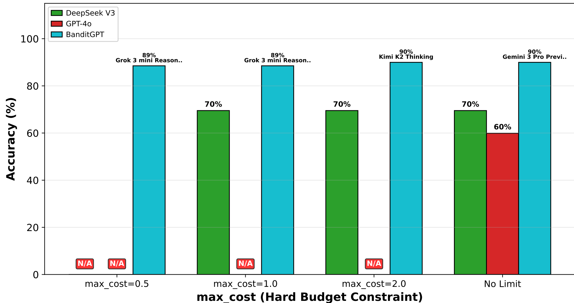
Figure 8: Constraint-Aware Routing (Standard Mode, \lambda=0 ) min_quality=70.0% | BanditGPT finds "Budget Specialists"
