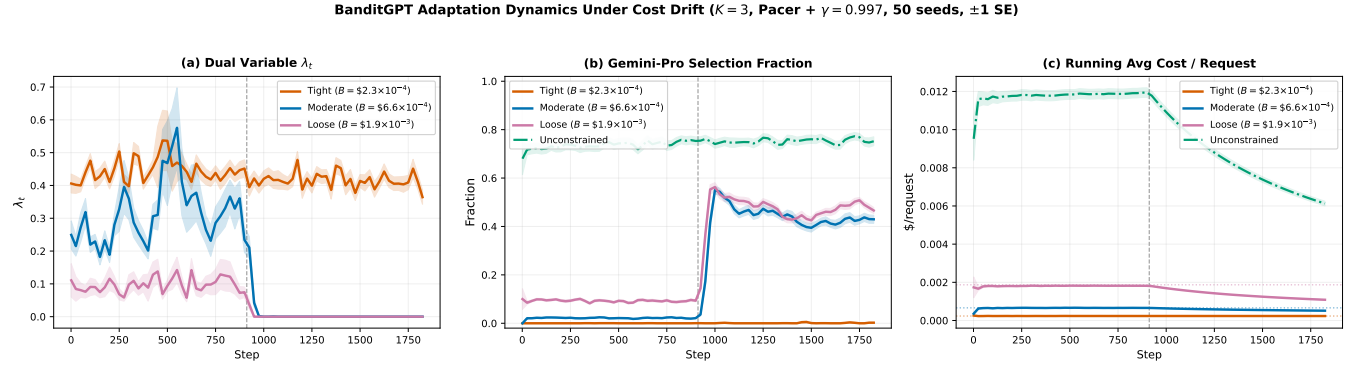
Figure 5: Adaptation Dynamics under Cost Drift. At t = 1000 , Gemini-2.5-Pro becomes significantly cheaper. BanditGPT detects the cost drop, lowers the dual penalty, and dynamically reroutes traffic to the higher-quality model while perfectly pacing the remaining budget.
