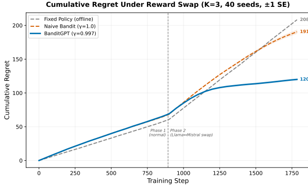
Figure 4: Cumulative Regret under Reward Drift. BanditGPT ( \gamma = 0.997 ) adapts rapidly to quality degradation, unlike naive bandits or frozen policies.
