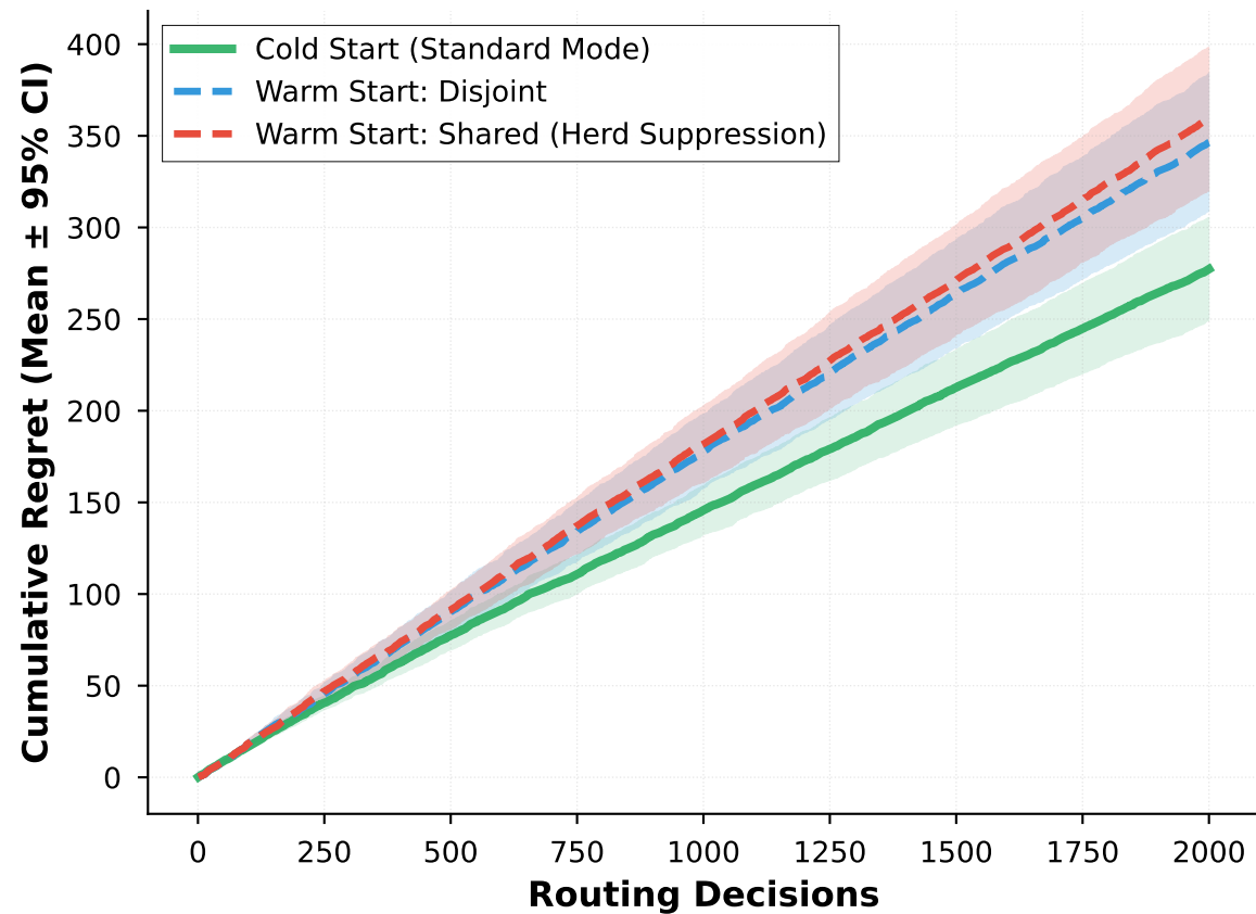
A) Regret Curves: Cold Start Outperforms Warm Start
