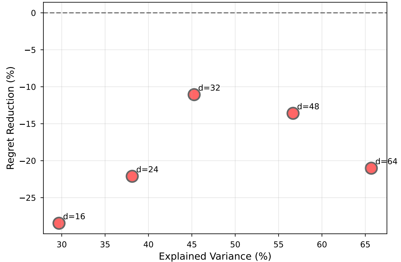
Signal vs. Generalization Trade-off
