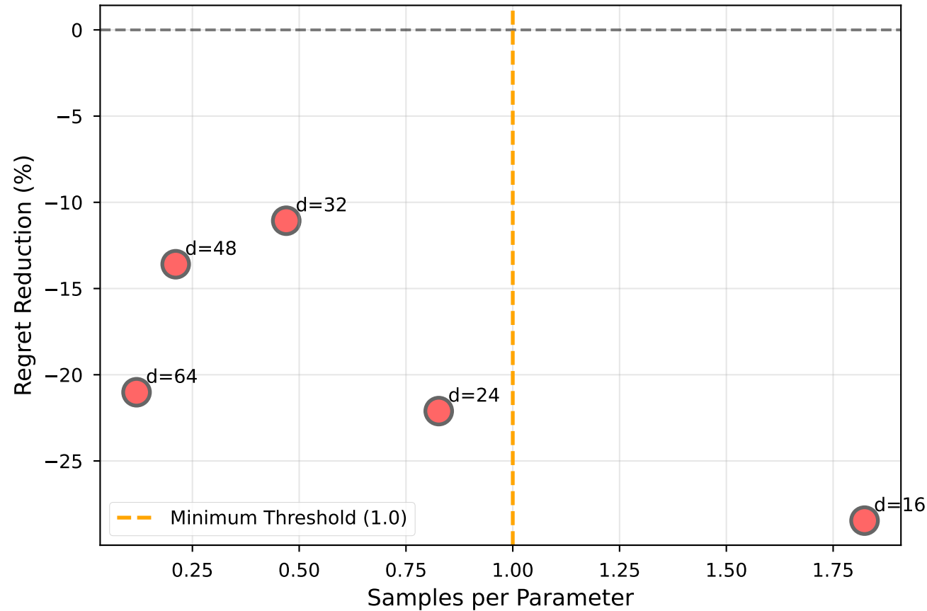
Sample Complexity Lower Bound
