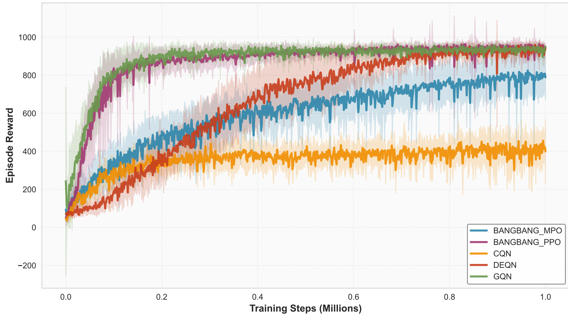
Walker Walk - Seed-Averaged Rewards
