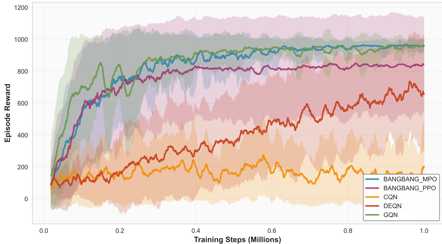
Reacher Easy - Smoothed Seed-Averaged Rewards (MA=20)
