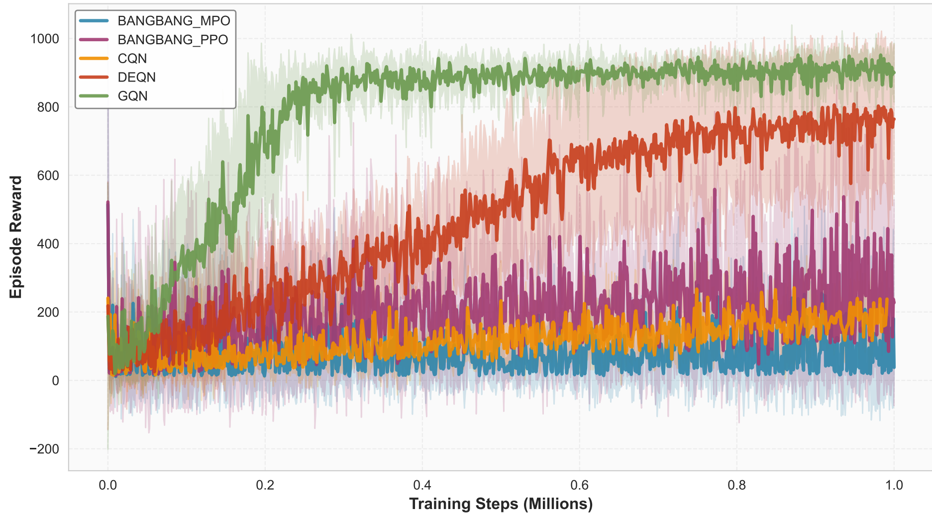
Quadruped Walk - Seed-Averaged Rewards
