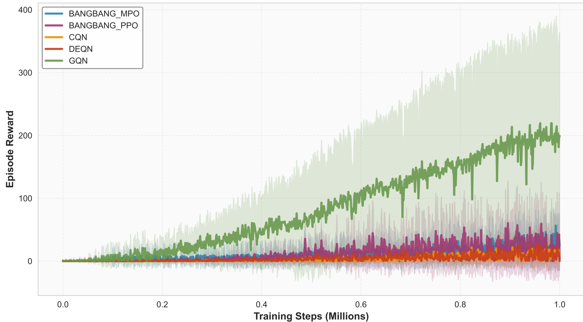
Hopper Hop - Seed-Averaged Rewards
