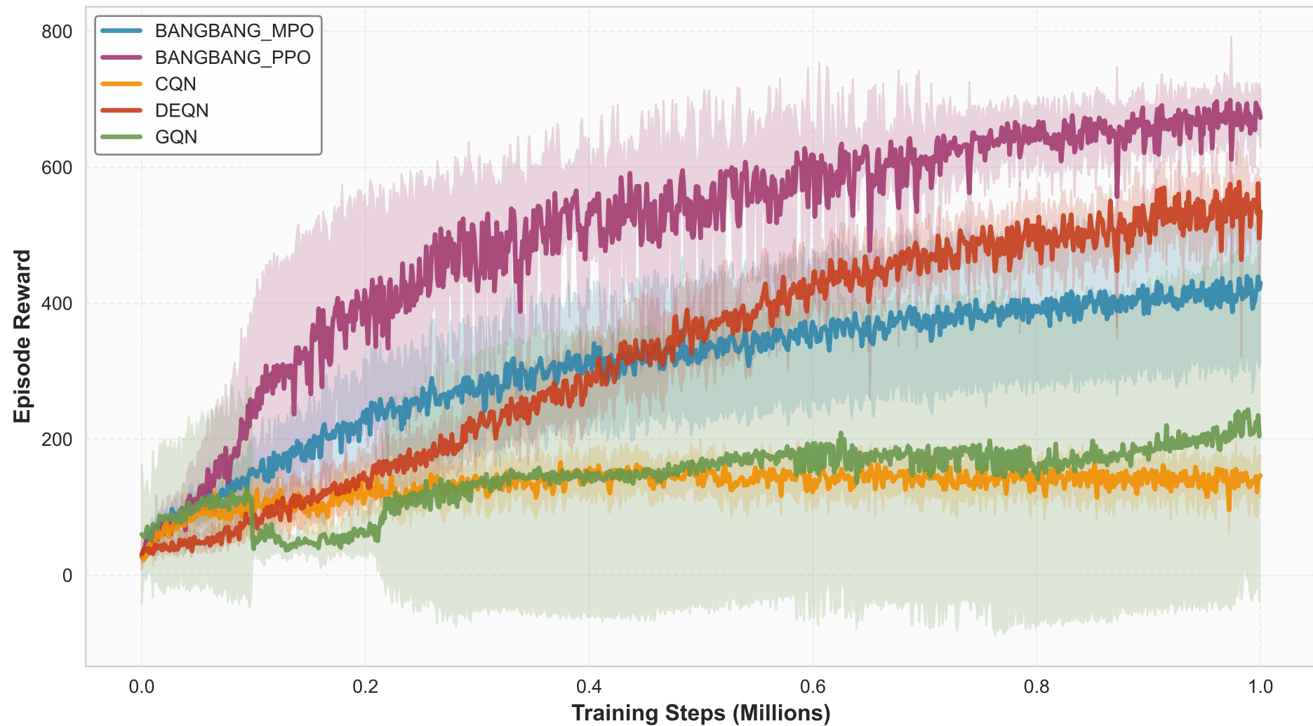
Walker Run - Seed-Averaged Rewards
