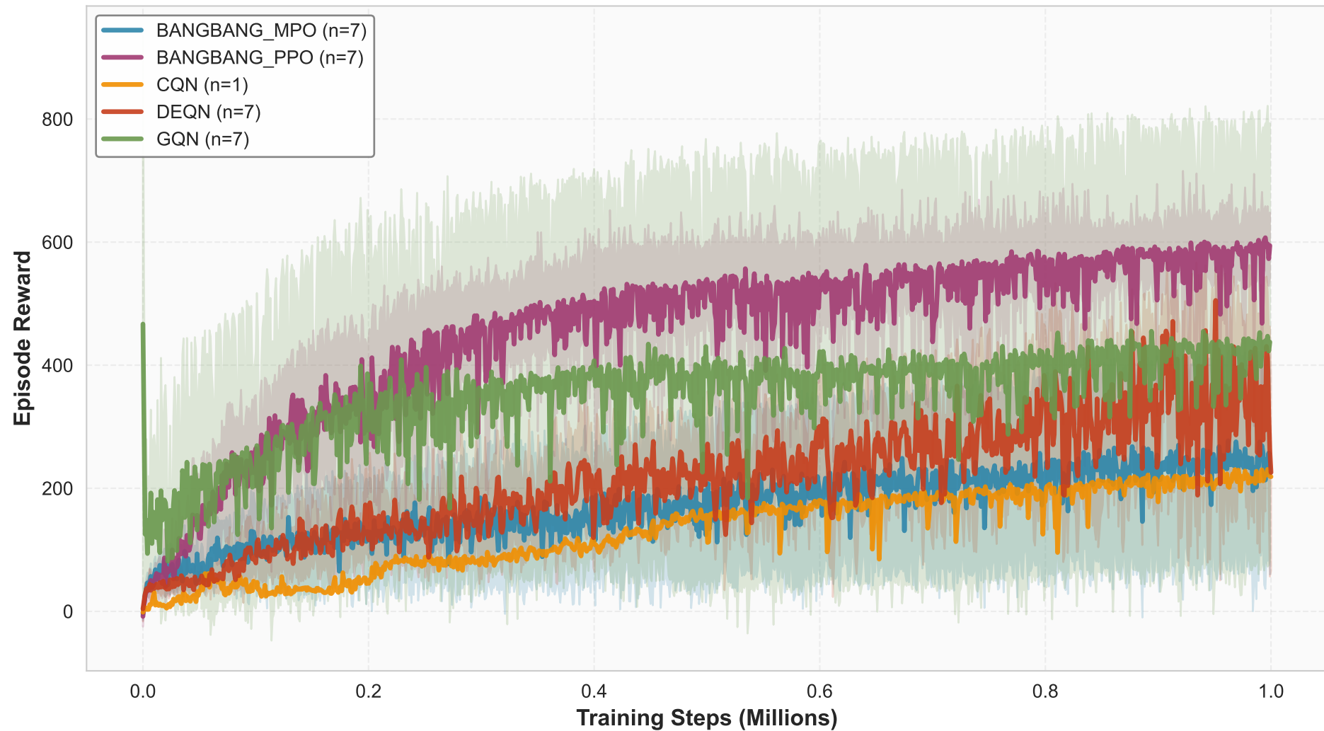
Cheetah Run - Seed-Averaged Rewards
