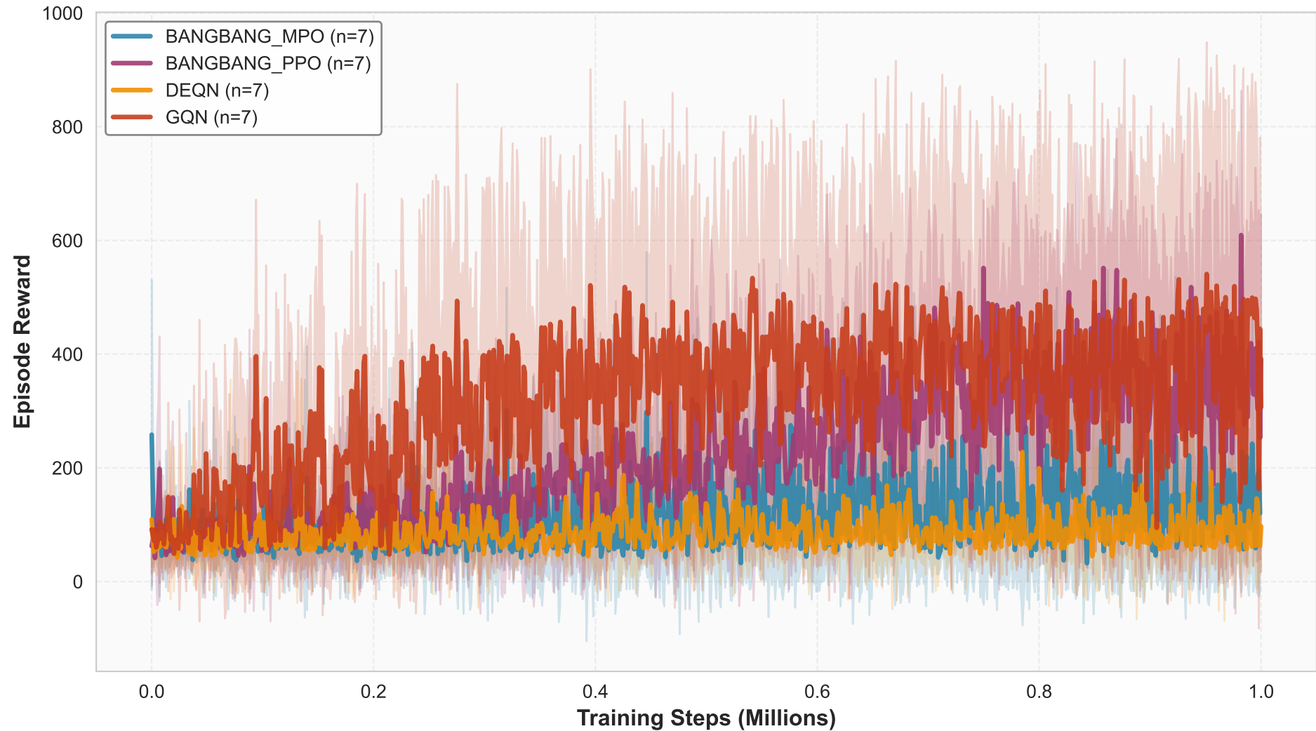
Fish Swim - Seed-Averaged Rewards
