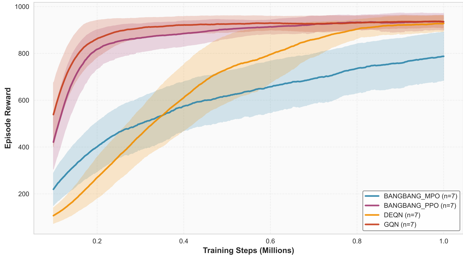
Walker Walk - Smoothed Seed-Averaged Rewards (MA=100)
