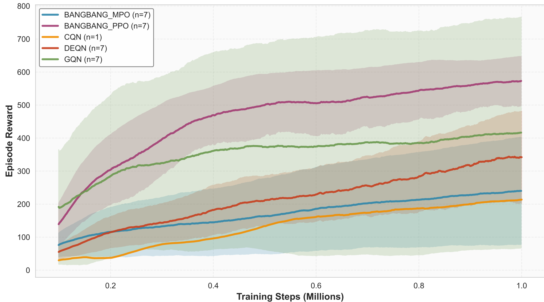
Cheetah Run - Smoothed Seed-Averaged Rewards (MA=100)
