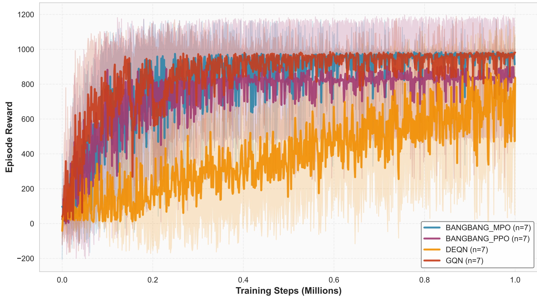
Reacher Easy - Seed-Averaged Rewards
