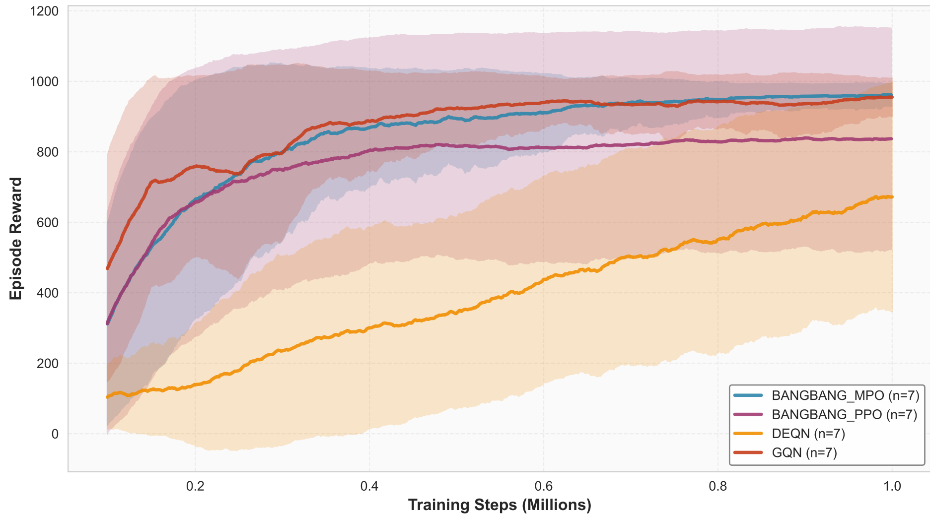
Reacher Easy - Smoothed Seed-Averaged Rewards (MA=100)
