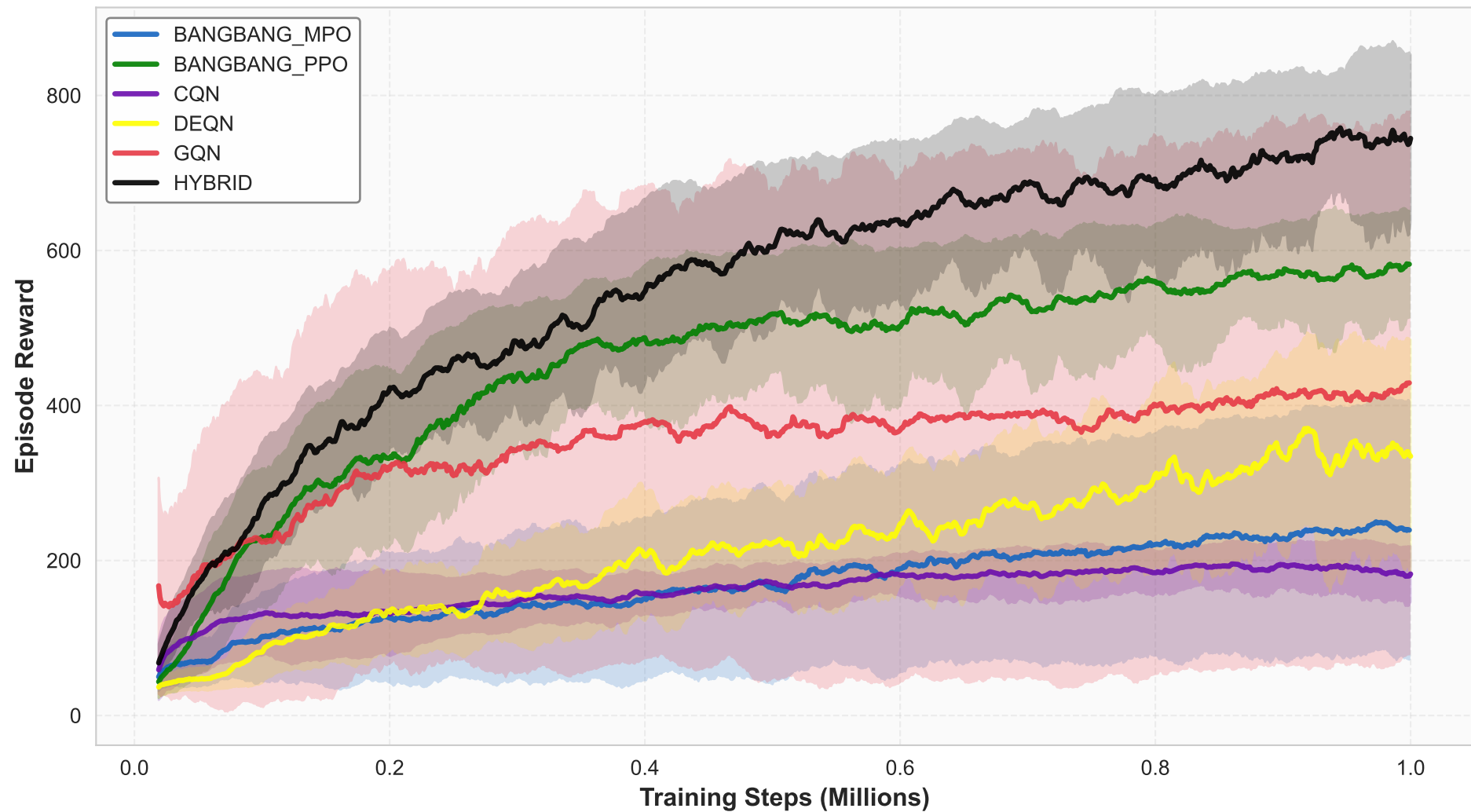
Cheetah Run - Smoothed Seed-Averaged Rewards (MA=20)
