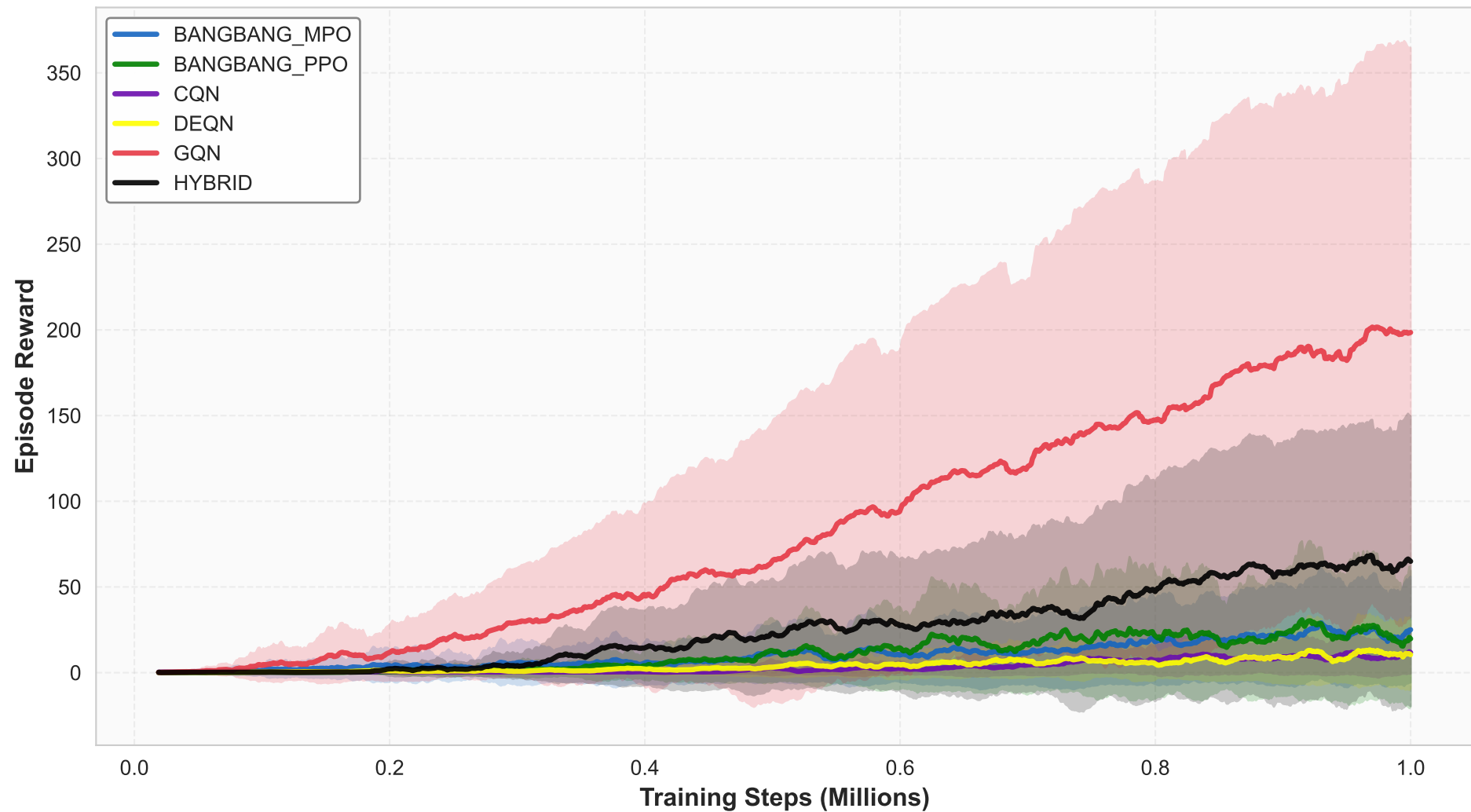
Hopper Hop - Smoothed Seed-Averaged Rewards (MA=20)
