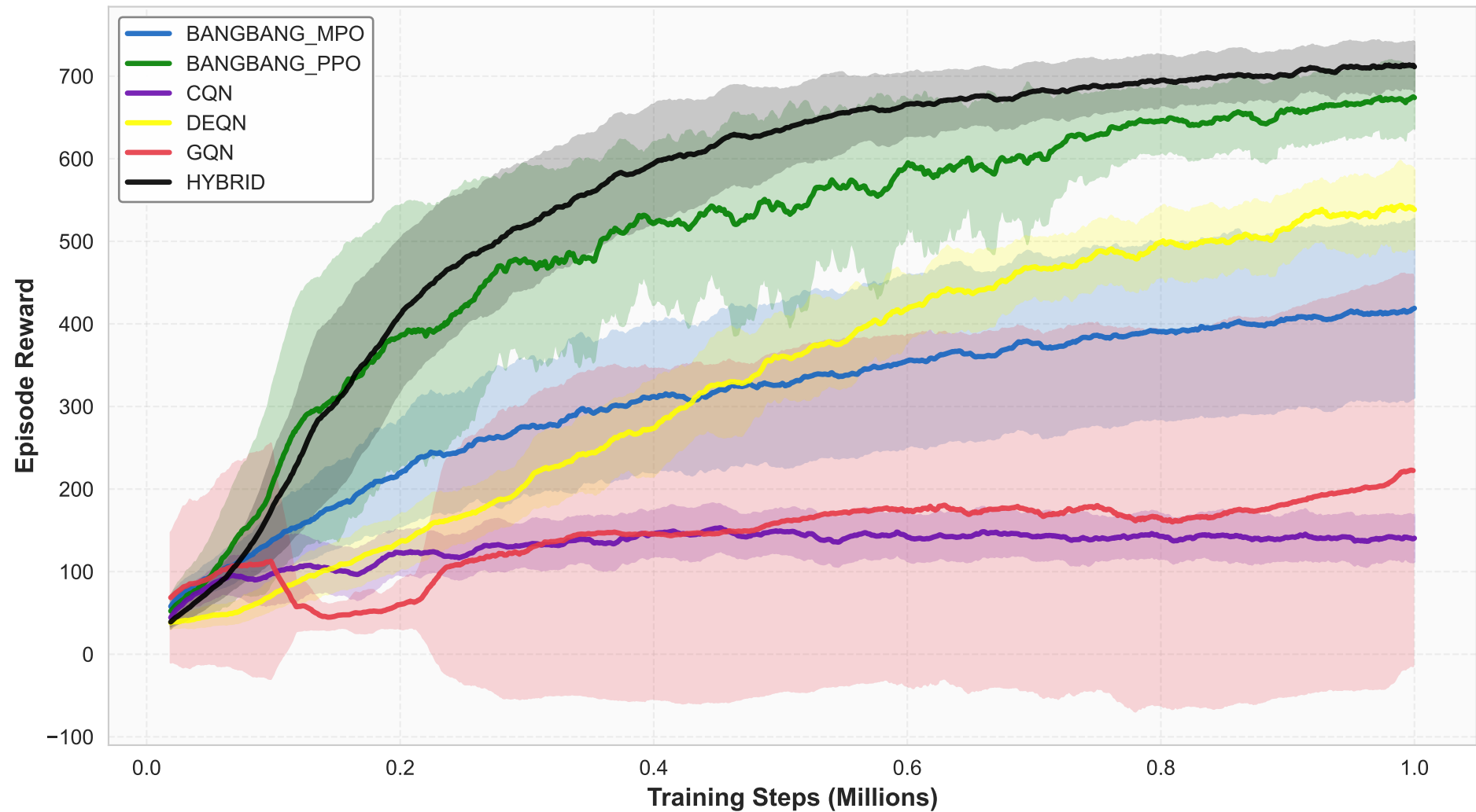
Walker Run - Smoothed Seed-Averaged Rewards (MA=20)
