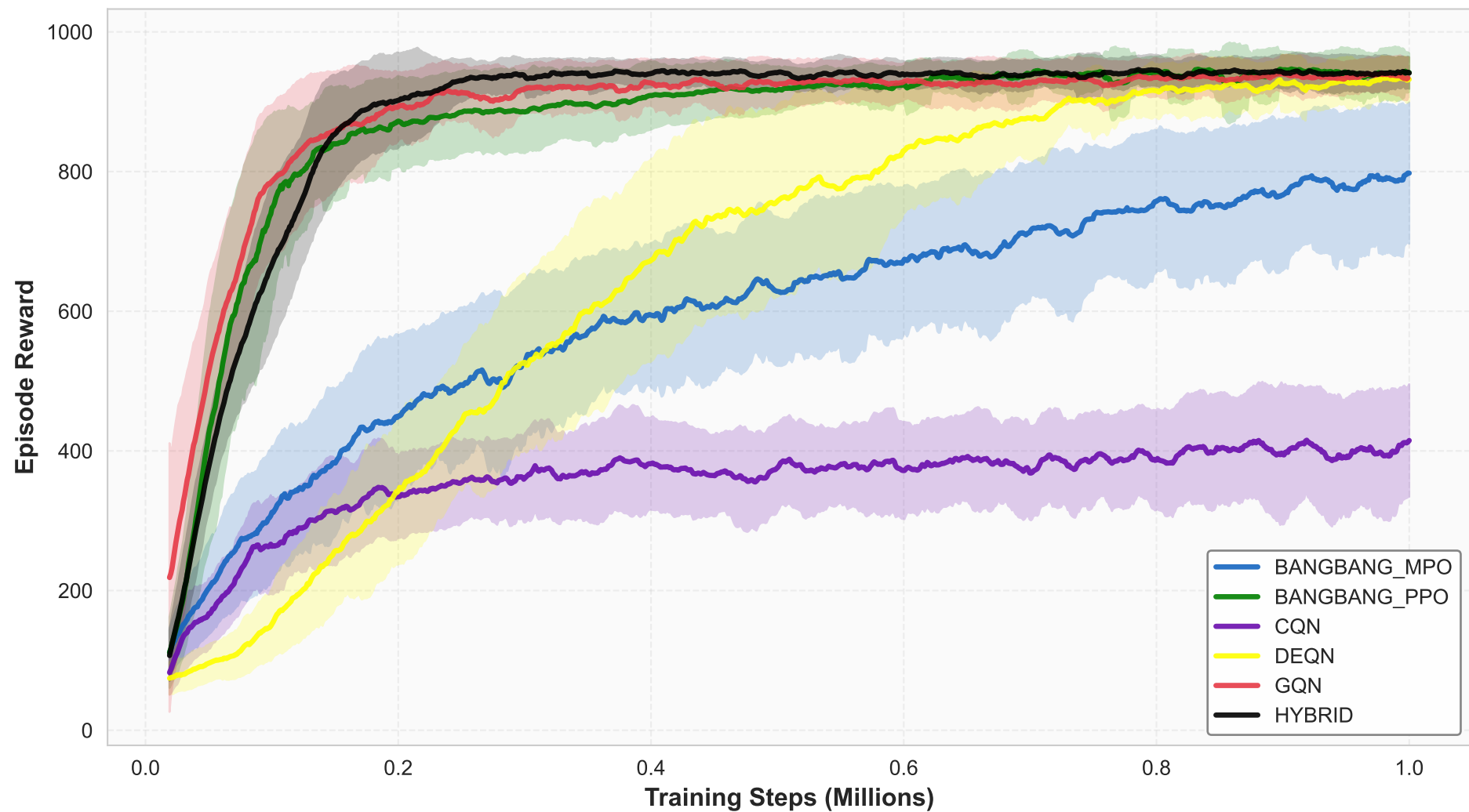
Walker Walk - Smoothed Seed-Averaged Rewards (MA=20)
