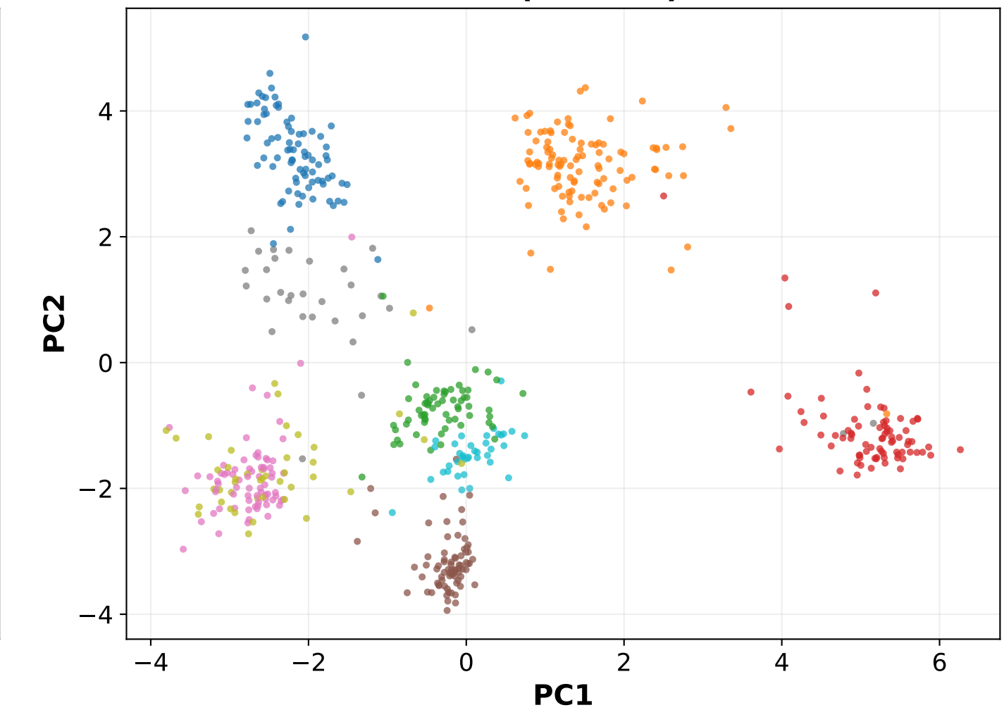
Self: SimCLR Silhouette (PCA-2D): 0.482
