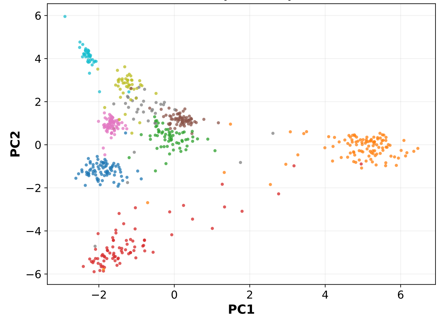
Self: VAE Silhouette (PCA-2D): 0.540
