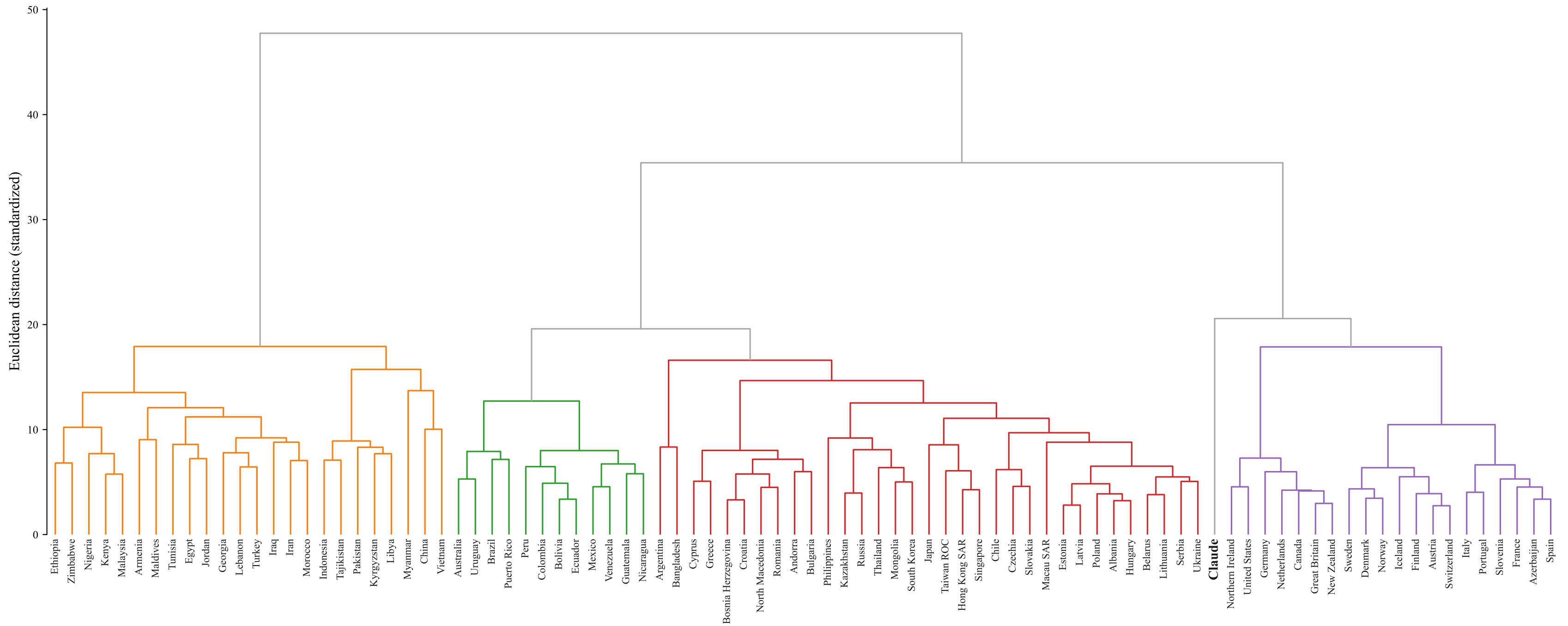
Hierarchical Clustering of Value Positions
