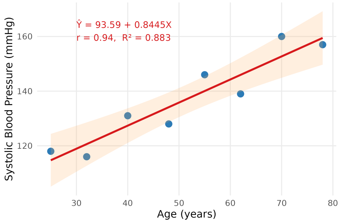
Figure 2: Scatter plot with fitted regression line: Age vs. Systolic Blood Pressure
