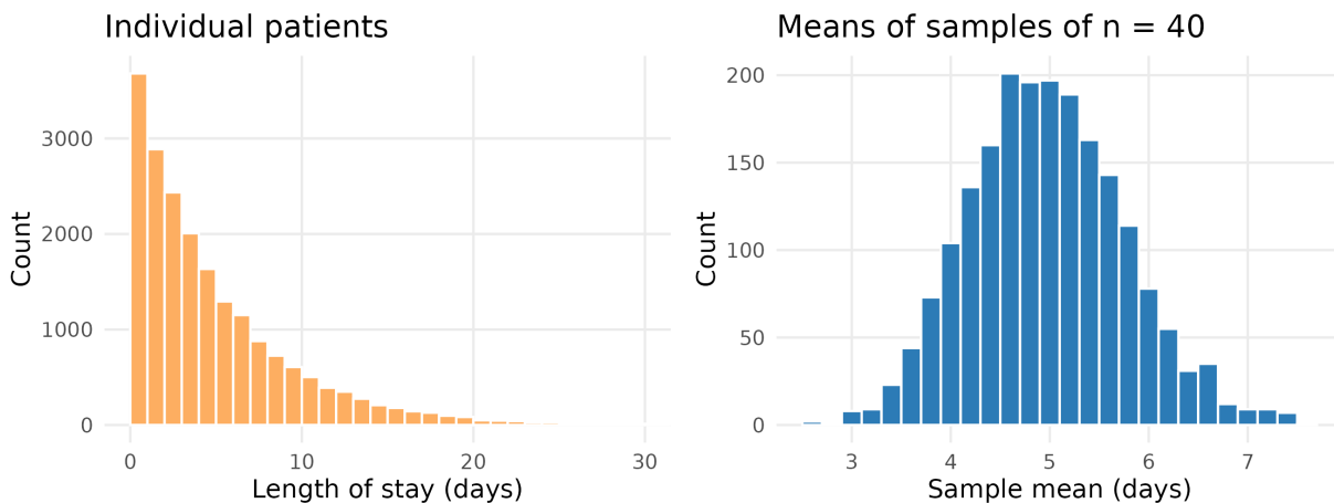
Figure 1: Left: length of stay of individual patients is right-skewed. Right: the means of many samples of 40 patients are approximately normal.
