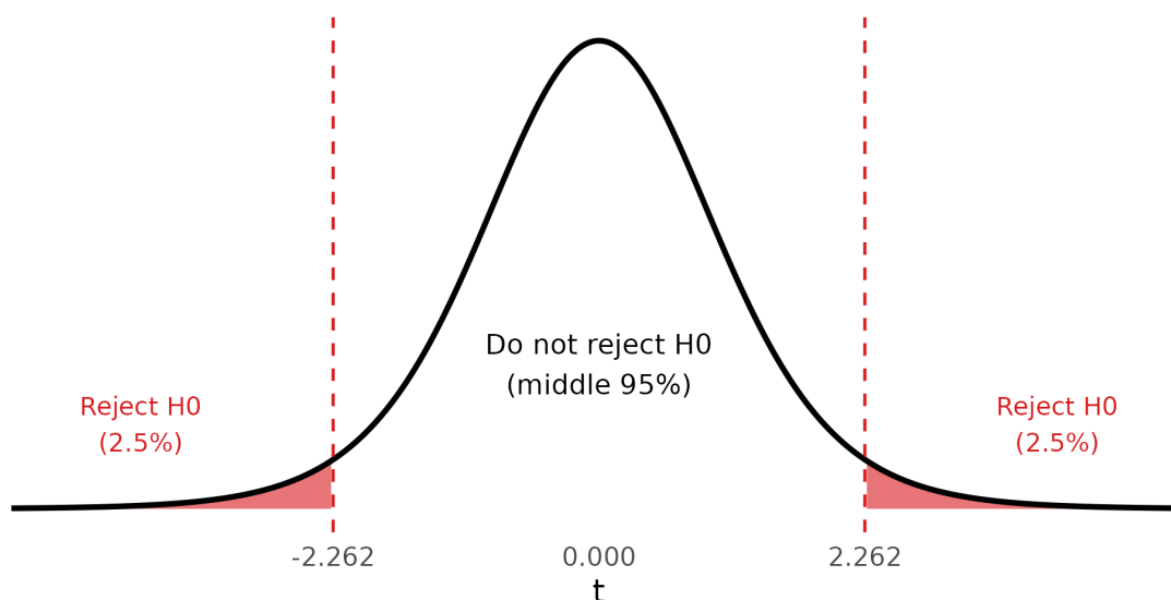
Figure 1: Two-tailed test at \alpha = 0.05 with df = 9 : reject H_0 when the test statistic falls in a red tail beyond the critical value 2.262
