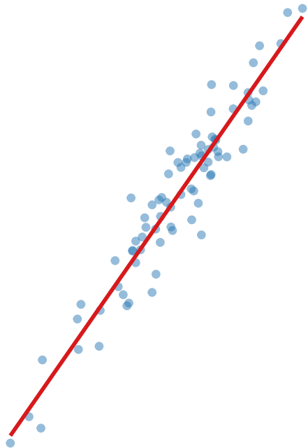
Strong positive
