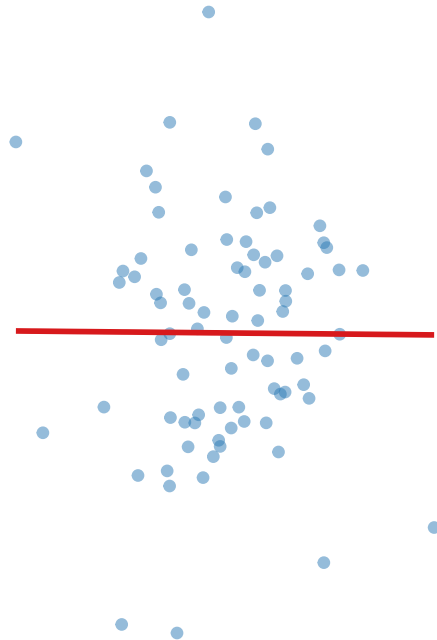
No relationship
