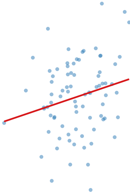
Weak positive
