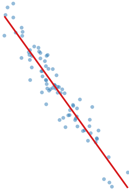
Strong negative
