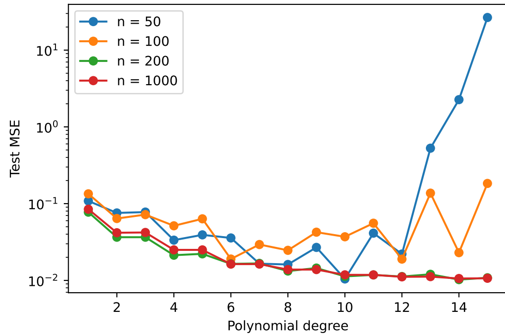
Effect of n ( \sigma = 0.1 )
