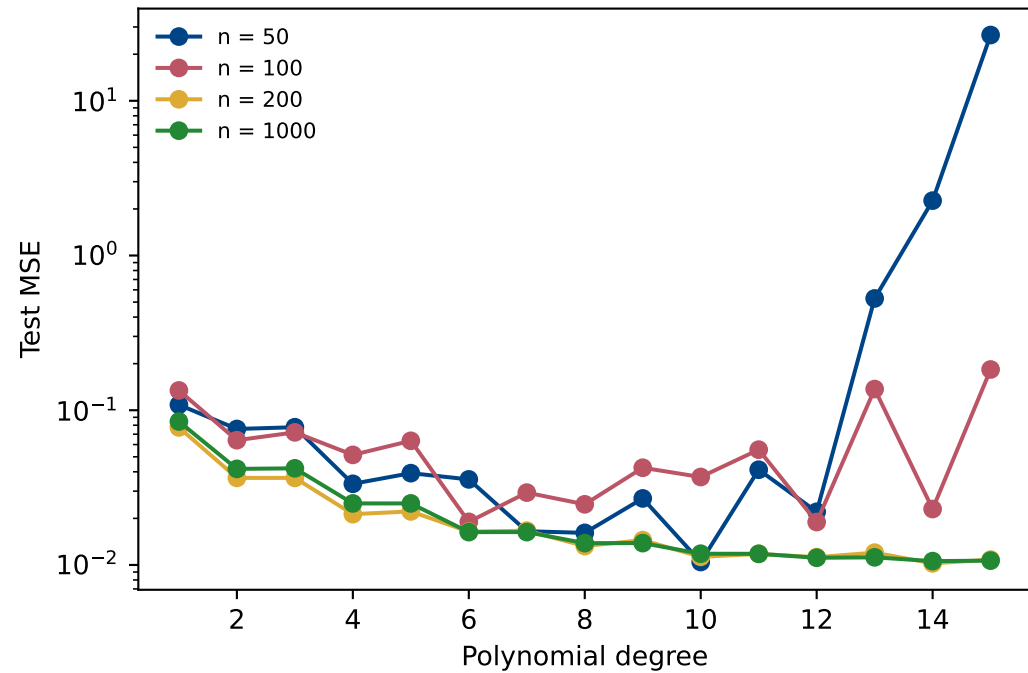
Effect of n ( \sigma = 0.1 )
