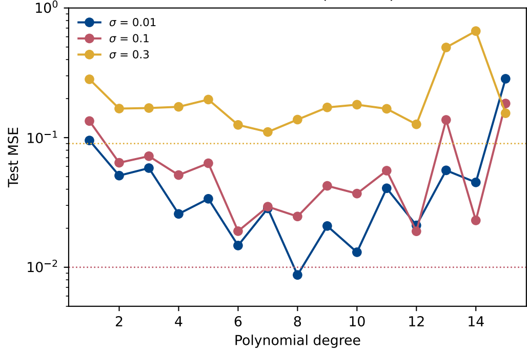
Effect of noise ( n = 100 )
