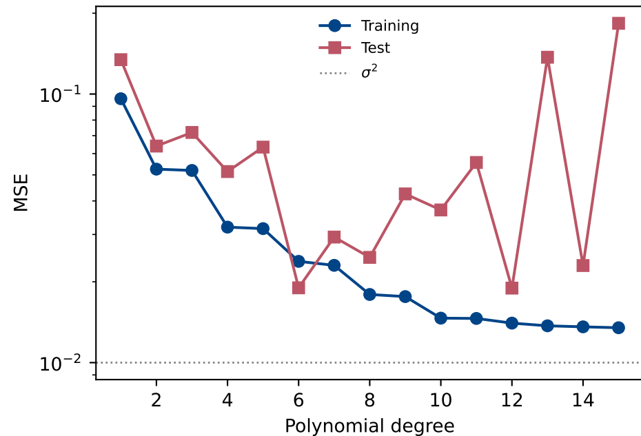
MSE vs polynomial degree
