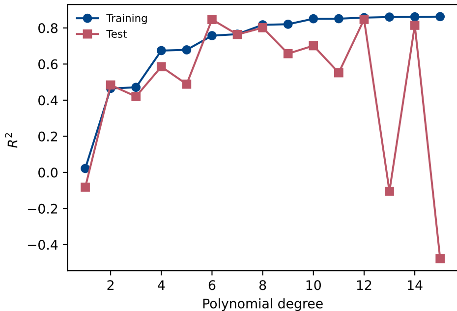
R^2 vs polynomial degree
