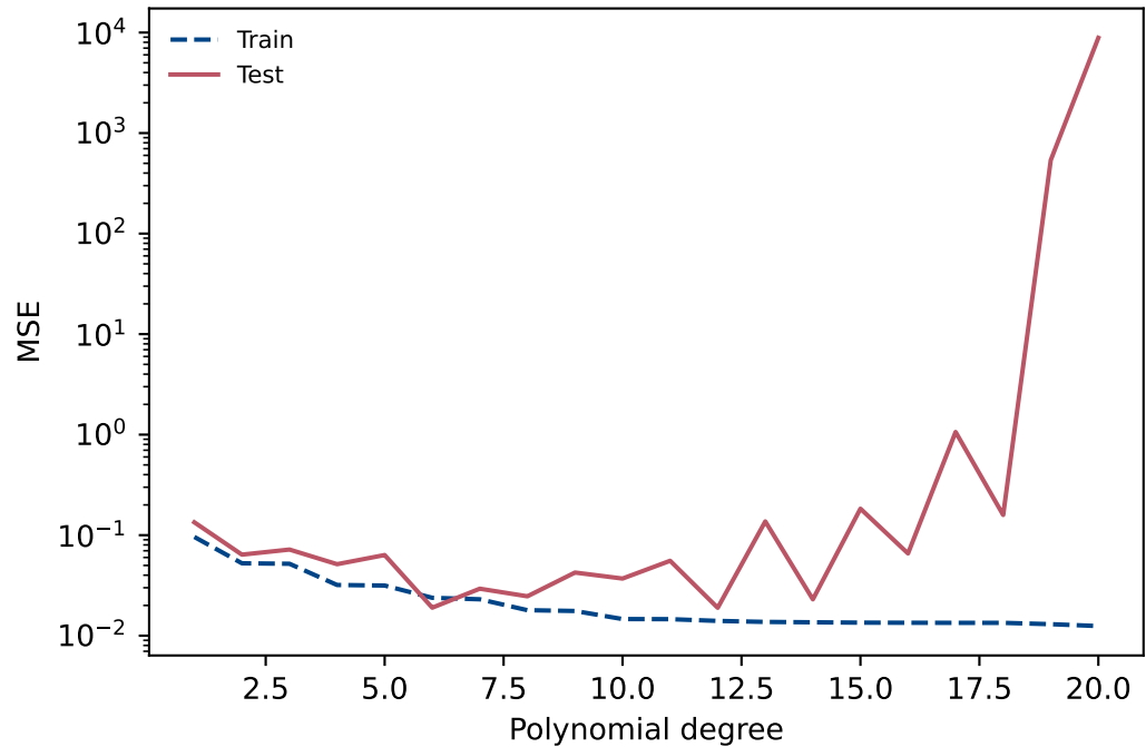
Train vs test MSE ( n = 100 )
